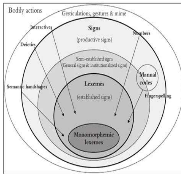
Figure 1: A hierarchy of lexicalization in signed languages
